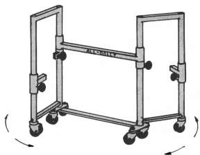
Patented Pivoting leg design
